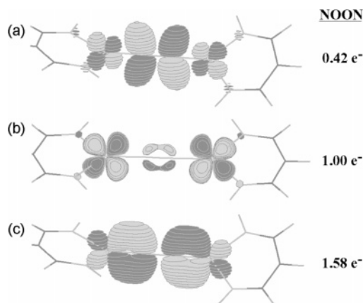
Figure 12. Key frontier orbitals from the MCSCF calculations on L'FeNNFeL' . Orbital (a) has 48% Fe and 48% N character, (b) has 96% Fe and 2% N character, and (c) has 60% Fe and 35% N character. NOON = natural orbital occupation number.
