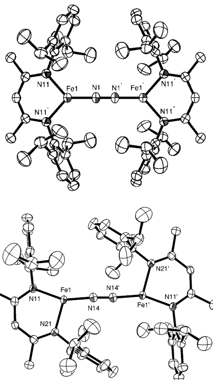
Figure 3. X-ray crystal structures of L^{\text{Me}}\text{FeNNFeL}^{\text{Me}} . Top: pentane solvate in C2/m ( 1a ). Bottom: solvent-free crystal in P2_1/n ( 1b ). Thermal ellipsoids shown at 50% probability, hydrogen atoms omitted for clarity. Selected bond lengths (Å) and angles (°): Fe–N( \text{N}_2 ) 1.745(3) in 1a , 1.775(2) in 1b ; Fe–N(diketiminate) 1.949(2) in 1a , 1.945(2) (N11) and 1.984(2) (N21) in 1b ; N–N 1.186(7) in 1a , 1.172(5) in 1b ; N( \text{N}_2 )–Fe–N(diketiminate) 130.75(6) in 1a , 155.5(1) (N11) and 109.5(1) (N21) in 1b ; N(diketiminate)–Fe–N(diketiminate) 97.6(1) in 1a , 94.8(1) in 1b .
