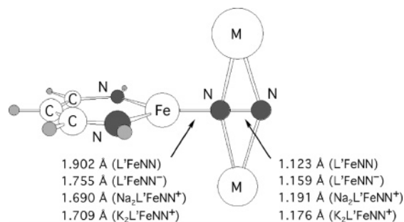
Figure 11. B3LYP/CZDZ*** optimized geometries for quartet L^RFeNN , triplet L^RFeNN^- , triplet Na_2L^RFeNN^+ , and triplet K_2L^RFeNN^+ .
