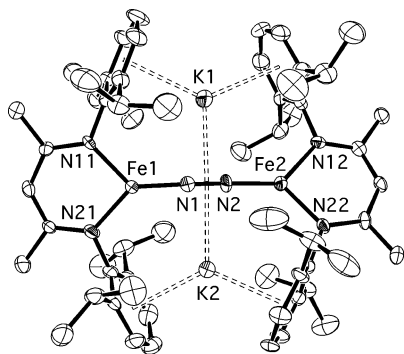
Figure 10. X-ray crystal structure of K_2L^{Me}FeNNFeL^{Me} . Thermal ellipsoids shown at 50% probability, hydrogen atoms omitted for clarity. Selected bond lengths (Å) and angles ( ^\circ ): Fe(1)–N(1) 1.741(5), Fe(1)–N(11) 1.915(5), Fe(1)–N(21) 1.936(5), Fe(2)–N(2) 1.736(5), Fe(2)–N(12) 1.931(5), Fe(2)–N(22) 1.928(5), N(1)–N(2) 1.215(6), K(1)–N(1) 2.778(6), K(1)–N(2) 2.748(5), K(2)–N(1) 2.800(6), K(2)–N(2) 2.796(5); N(11)–Fe(1)–N(21) 96.2(2), N(1)–Fe(1)–N(11) 131.3(2), N(1)–Fe(1)–N(21) 132.6(2), N(12)–Fe(2)–N(22) 95.0(2), N(2)–Fe(2)–N(12) 133.6(2), N(2)–Fe(2)–N(22) 131.0(2).
