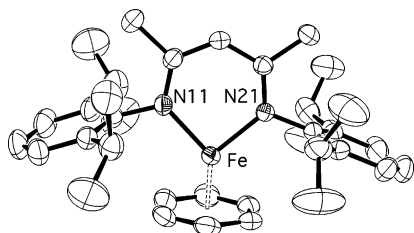
Figure 5. X-ray crystal structure of L^{\text{Me}}\text{Fe}(\text{C}_6\text{H}_6) . Thermal ellipsoids shown at 50% probability, hydrogen atoms omitted for clarity. Bond lengths (Å) and angles ( ^\circ ): Fe–N(11) 1.966(1), Fe–N(21) 1.981(1), Fe–C 2.143(2), 2.139(2), 2.151(2), 2.157(2), 2.144(2), 2.143(2); N(11)–Fe(1)–N(21) 92.20(5).
