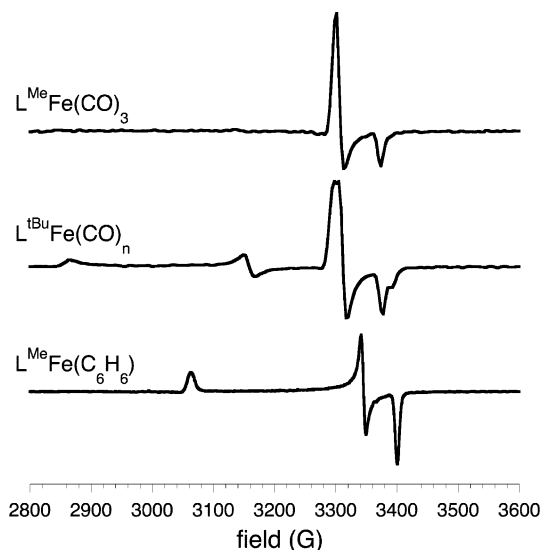
Figure 7. X-band EPR spectra of (a) L^{\text{Me}}\text{Fe}(\text{CO})_3 ; (b) a mixture of L^{\text{tBu}}\text{Fe}(\text{CO})_2 and L^{\text{tBu}}\text{Fe}(\text{CO})_3 ; (c) L^{\text{Me}}\text{Fe}(\text{C}_6\text{H}_6) . Solvent: toluene; temperature = 77 K; frequency = 9.42 GHz; power = 1.0 mW; attenuation = 30 dB.
